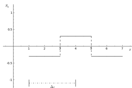
(c) S_3(x) .
