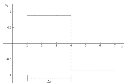
(a) S_1(x) .
