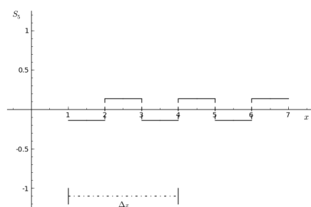
(e) S_5(x) .
