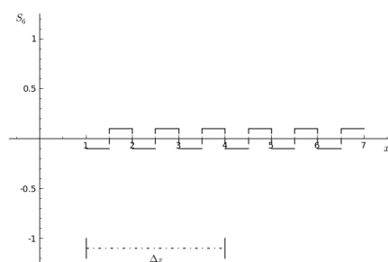
(f) S_6(x) .
